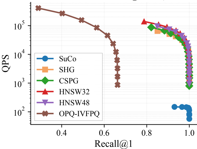
SIFT10M — Recall@1 vs QPS
