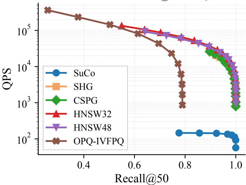
SIFT10M — Recall@50 vs QPS
