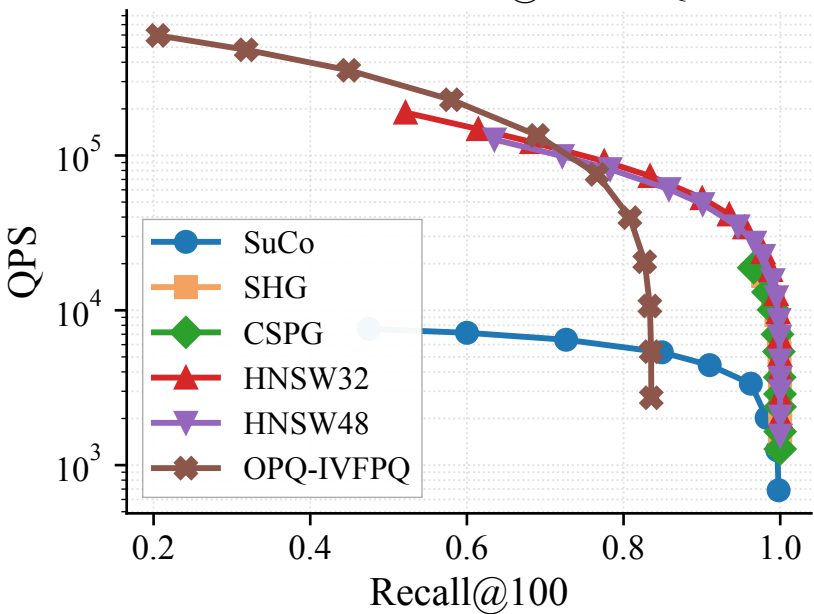
SIFT1M — Recall@100 vs QPS
