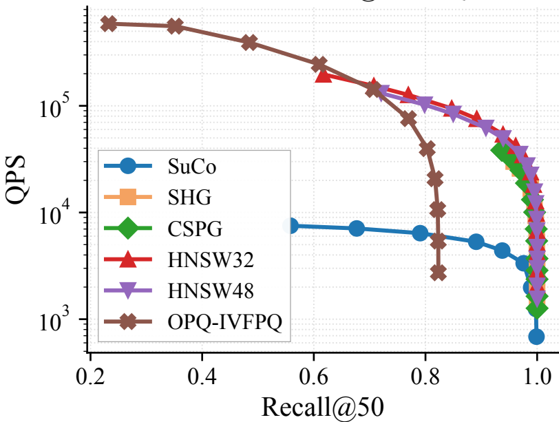
SIFT1M — Recall@50 vs QPS
