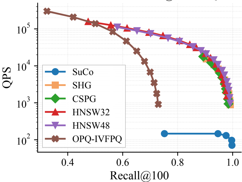
SPACEV10M — Recall@100 vs QPS
