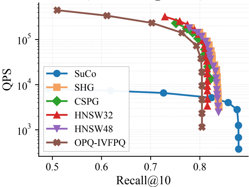
UQ-V — Recall@10 vs QPS
