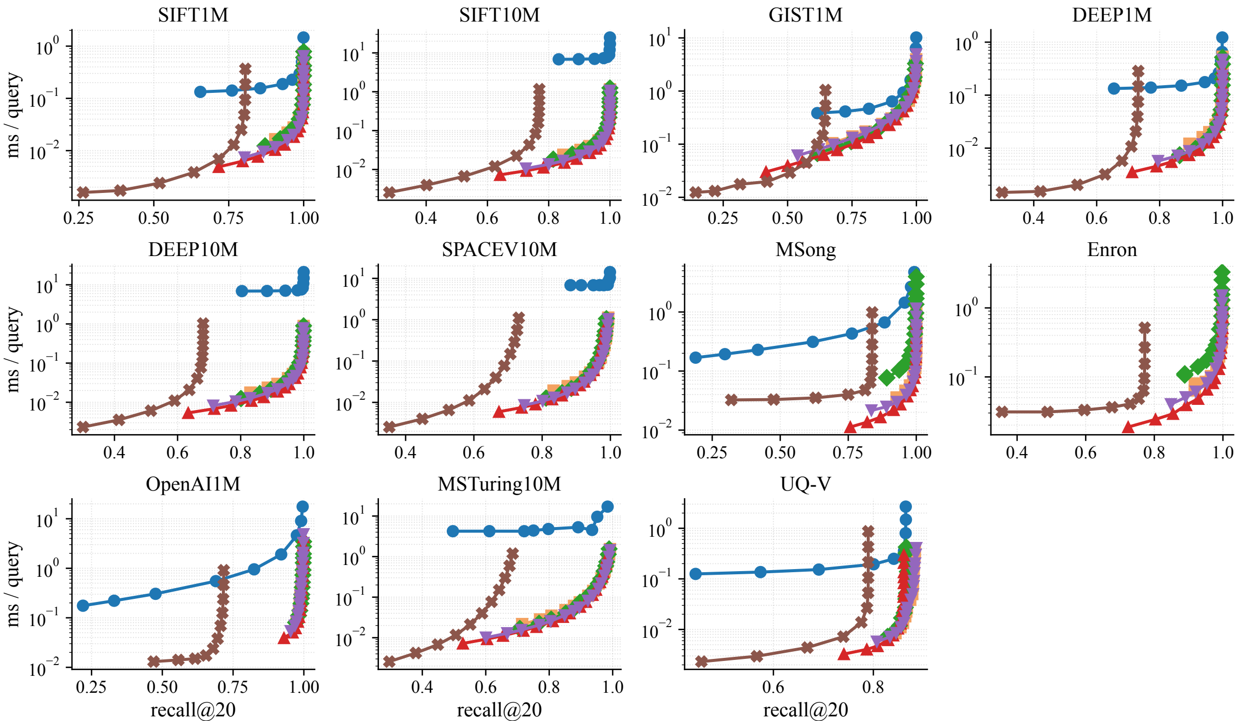
ms/query vs recall@20 (log-y)
