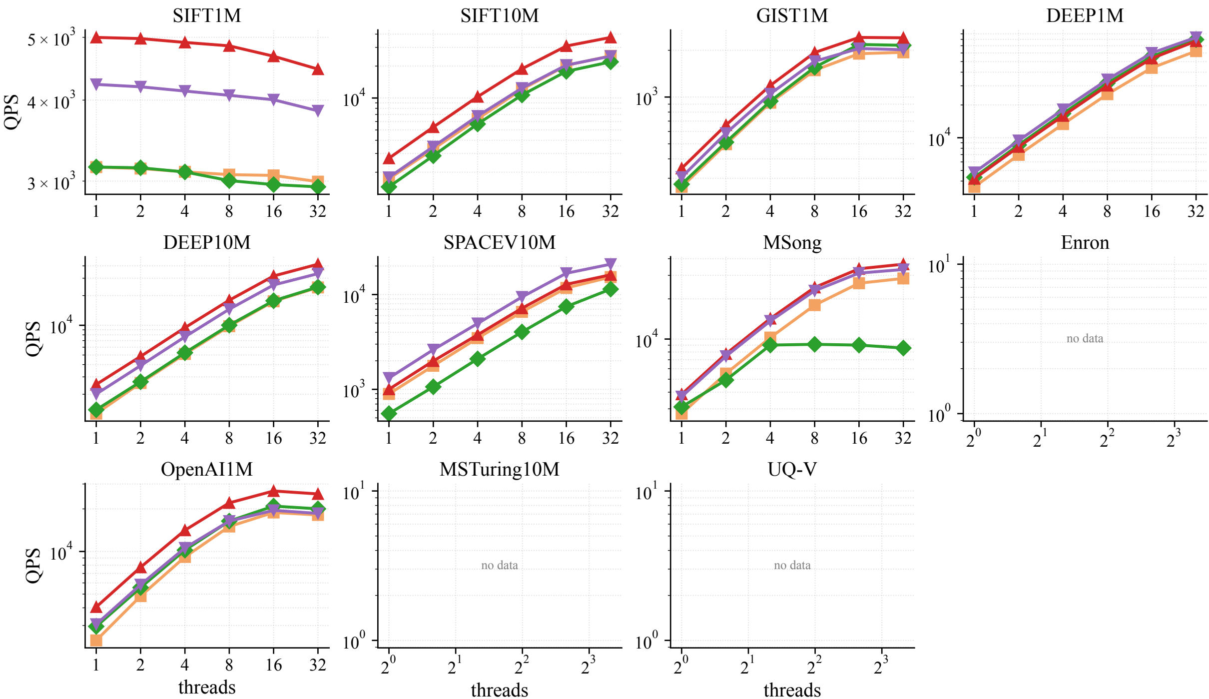
Thread-scaling: QPS vs threads @ recall \geq 0.95 (k=10)
