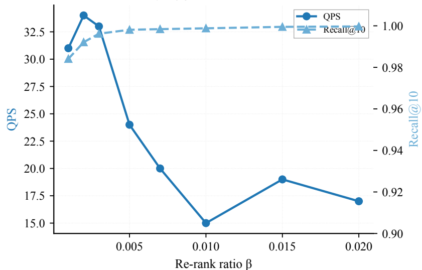
(b) Varying \beta ( \alpha=0.05 , SIFT10M)
