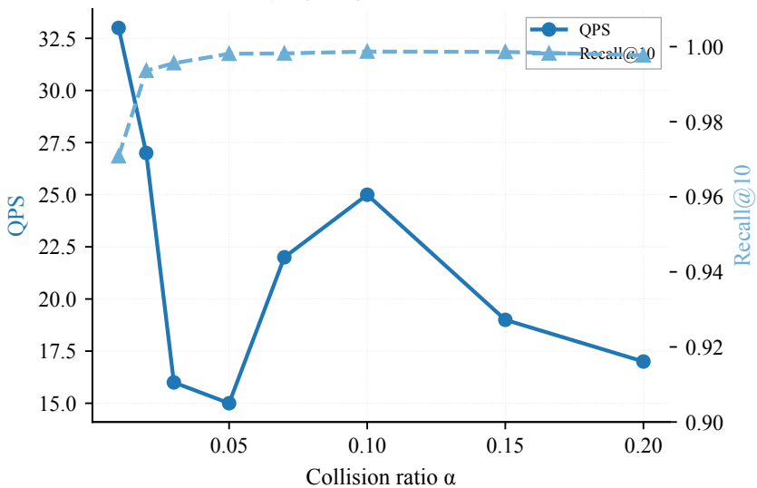
(a) Varying \alpha ( \beta=0.005 , SIFT10M)
