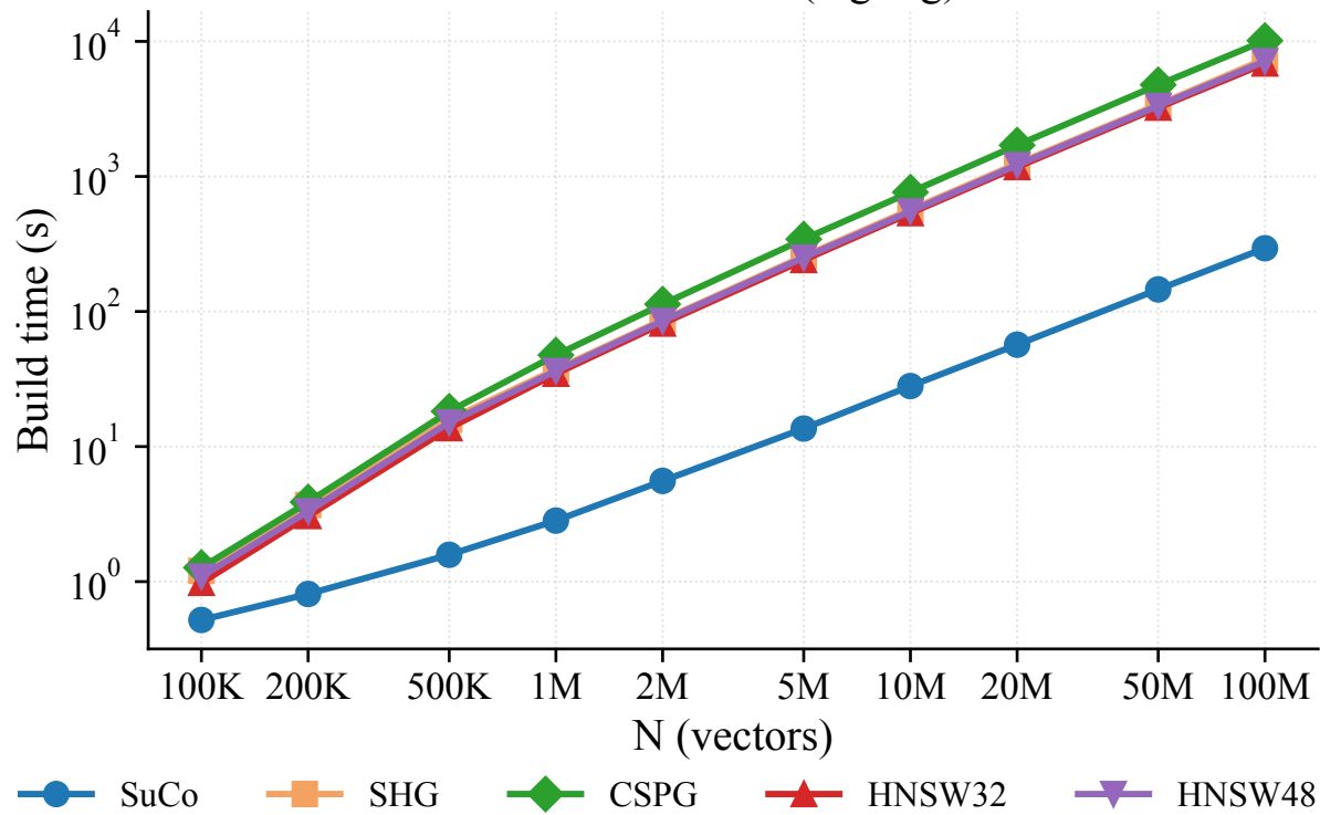
Build time vs N (log-log)
