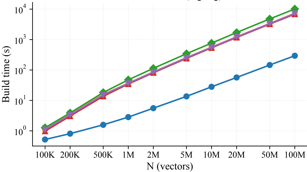
Build time vs N (log-log)
