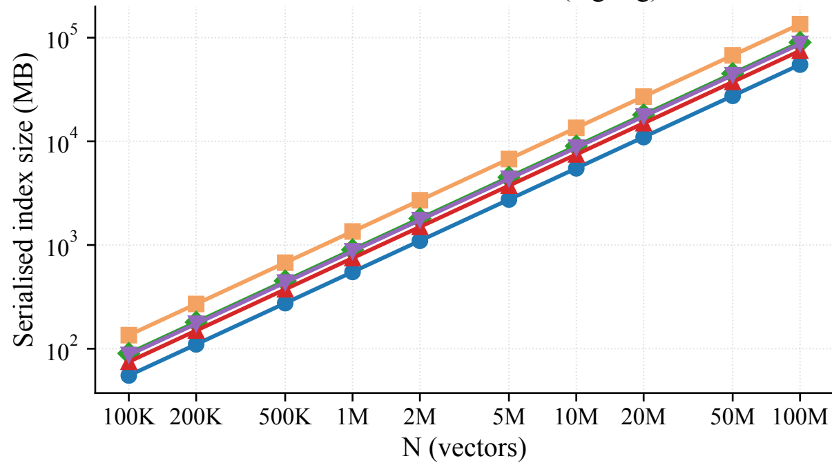
Serialised index size vs N (log-log)
