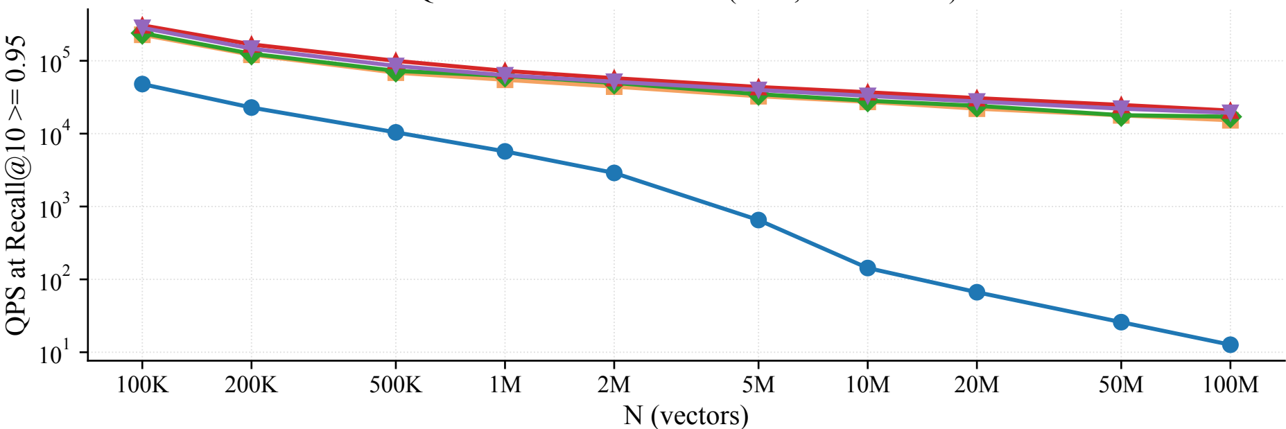
QPS at matched recall vs N ( k=10 , \text{recall} \geq 0.95 )
