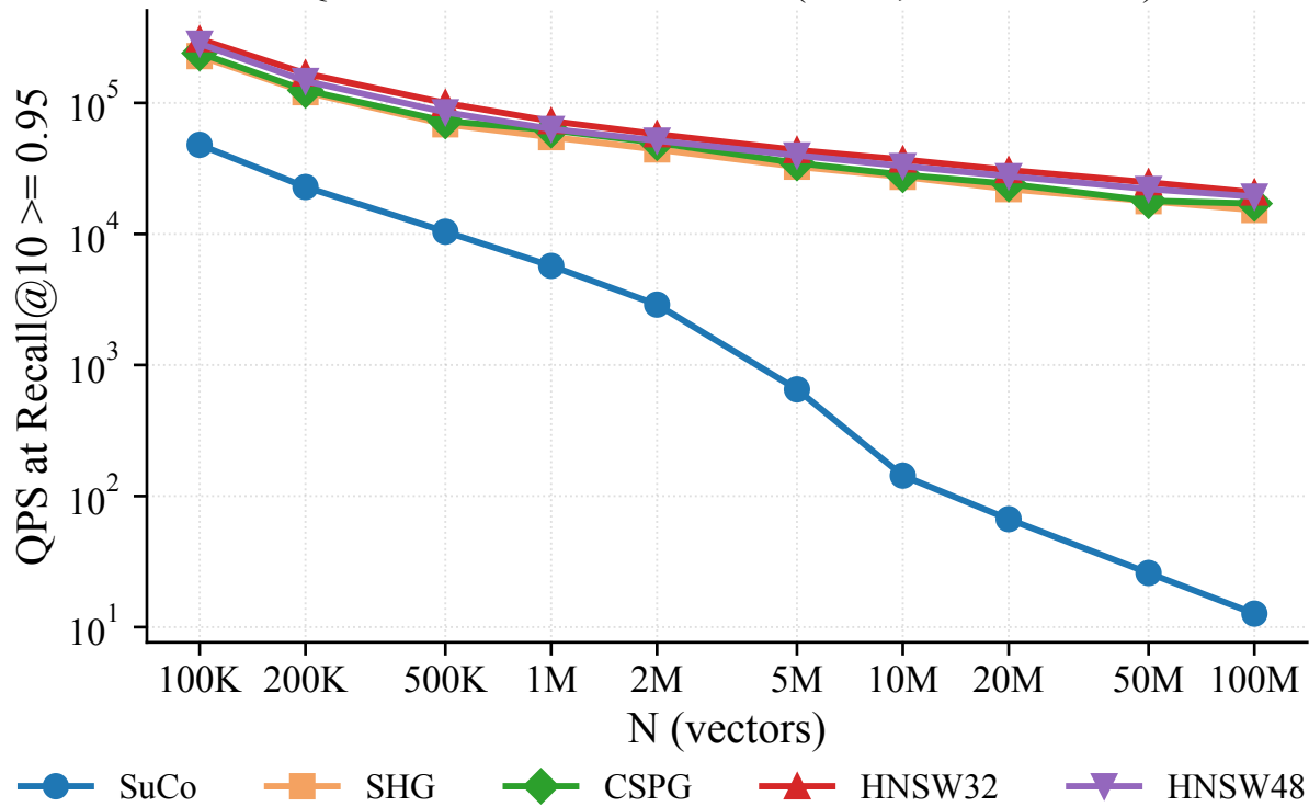
QPS at matched recall vs N (k=10, recall \geq 0.95 )
