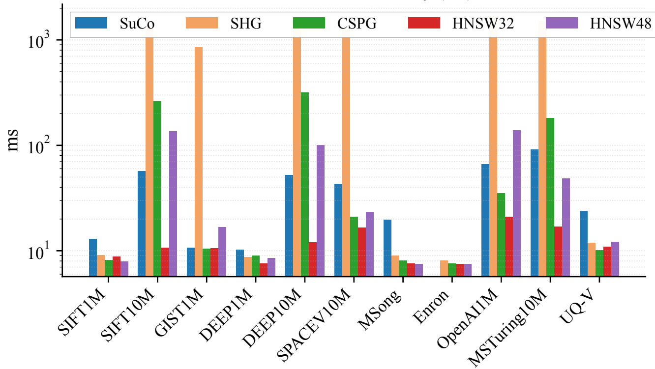
Cold-cache mean latency (ms)
