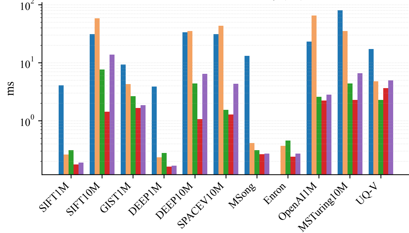
Warm-cache mean latency (ms)
