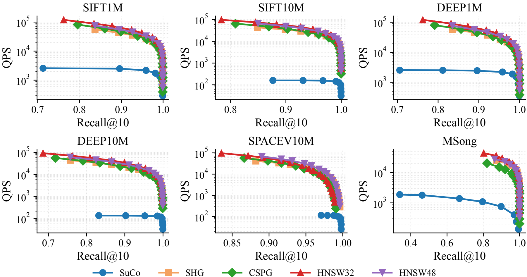
QPS vs Recall@10 — low-dimensional datasets
