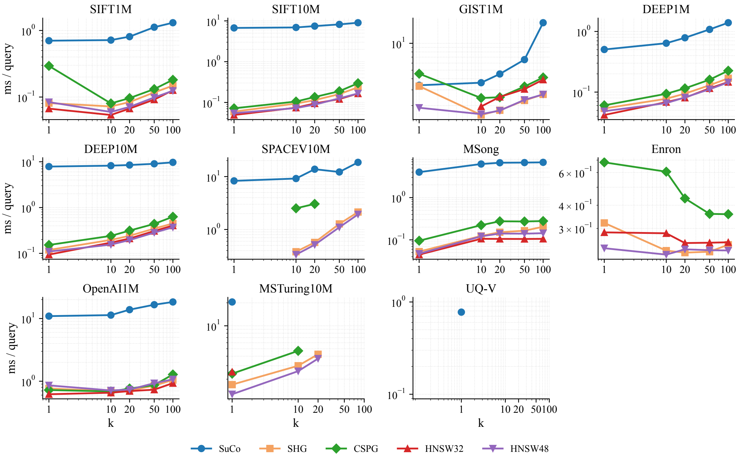
k sensitivity: ms/query at recall \geq 0.99
