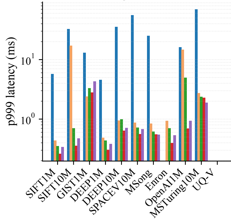
P999 @ recall 0.90
