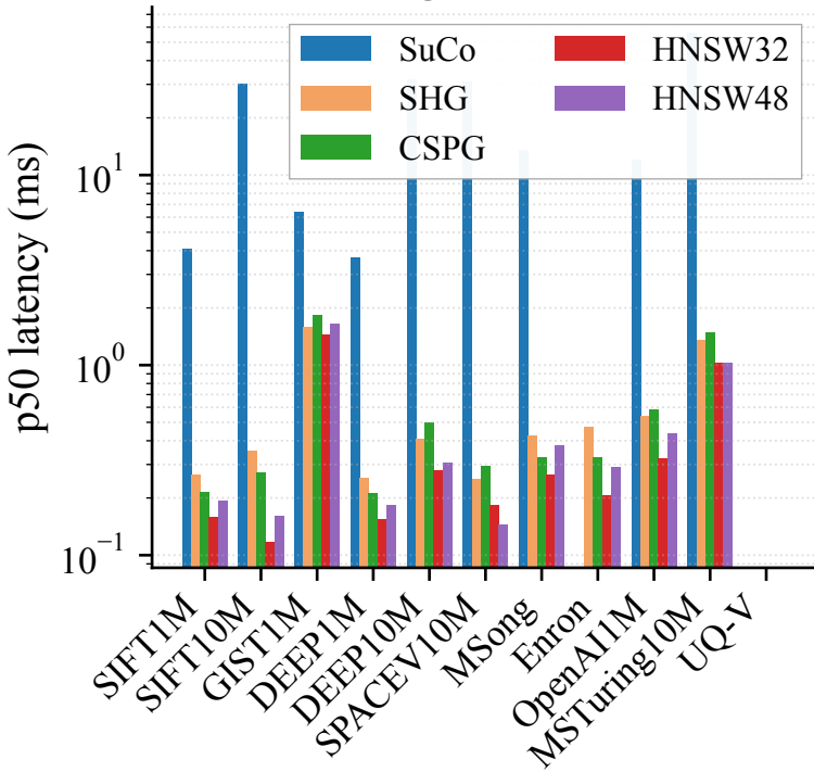
P50 @ recall 0.90
