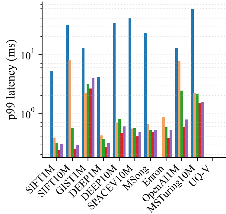
P99 @ recall 0.90
