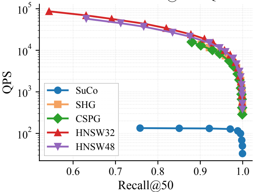
DEEP10M — Recall@50 vs QPS
