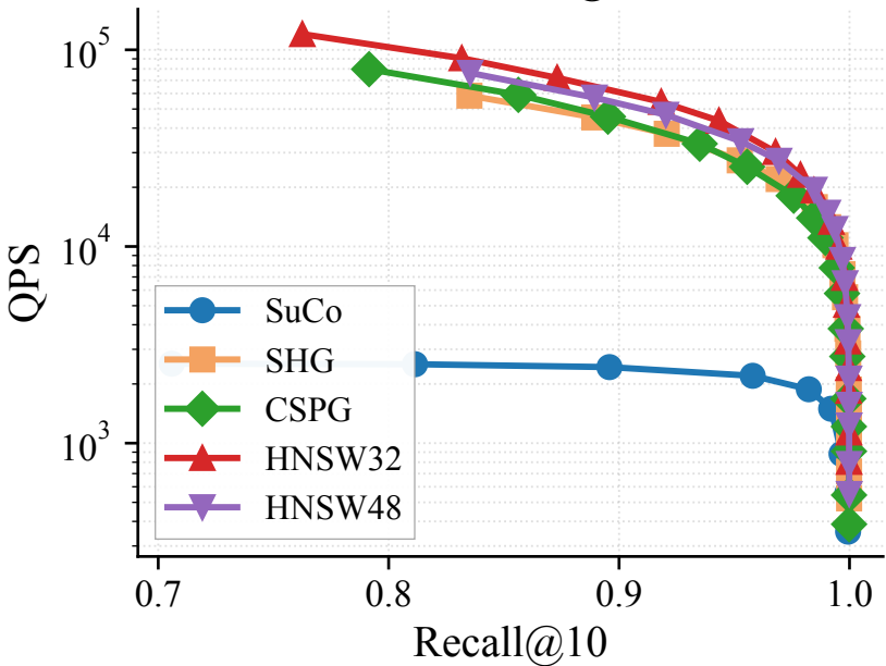
DEEP1M — Recall@10 vs QPS
