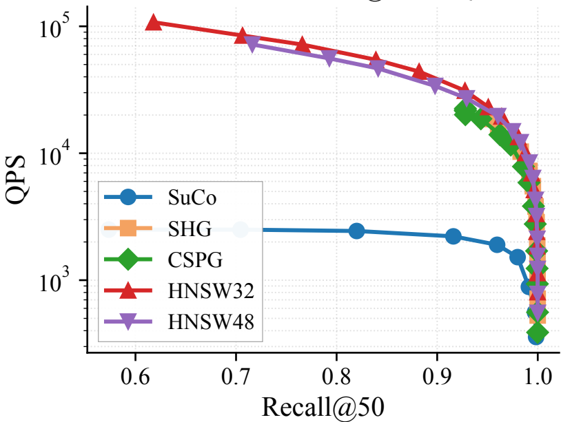
DEEP1M — Recall@50 vs QPS
