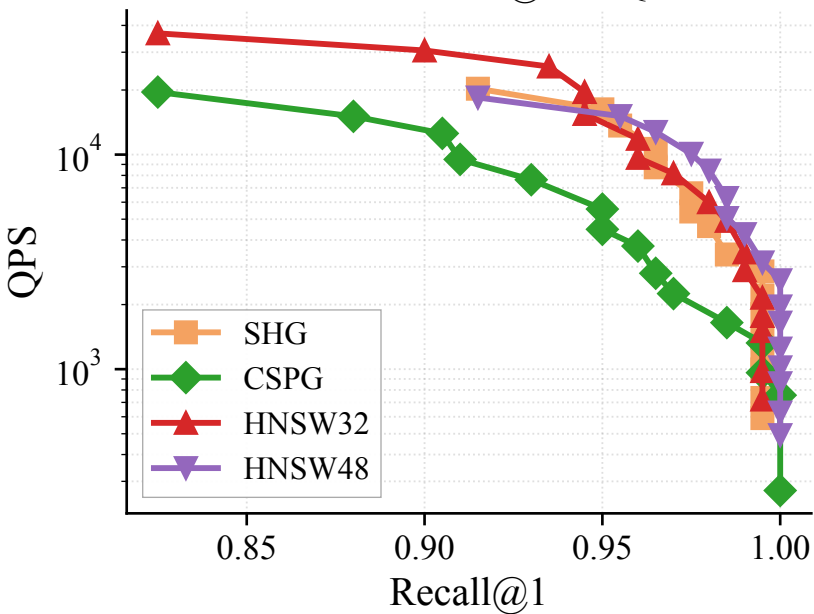
Enron — Recall@1 vs QPS
