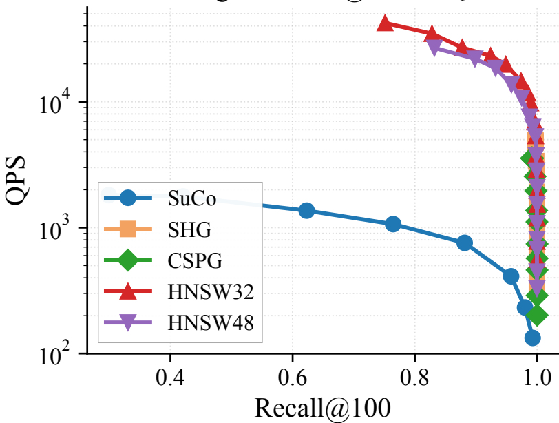
MSong — Recall@100 vs QPS
