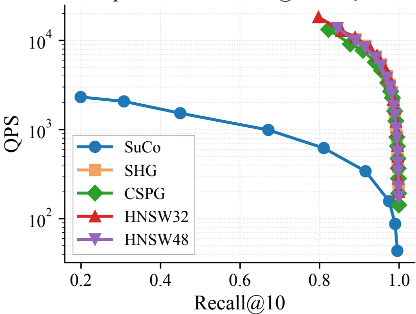
OpenAI1M — Recall@10 vs QPS
