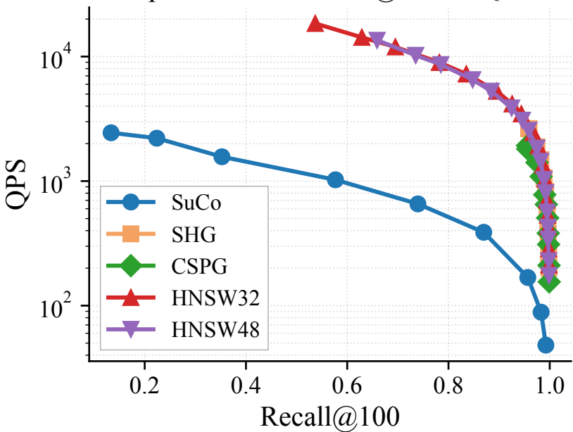
OpenAI1M — Recall@100 vs QPS
