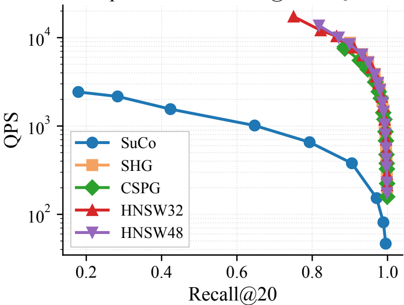
OpenAI1M — Recall@20 vs QPS
