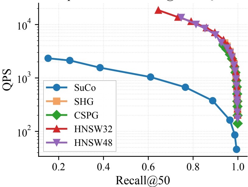
OpenAI1M — Recall@50 vs QPS
