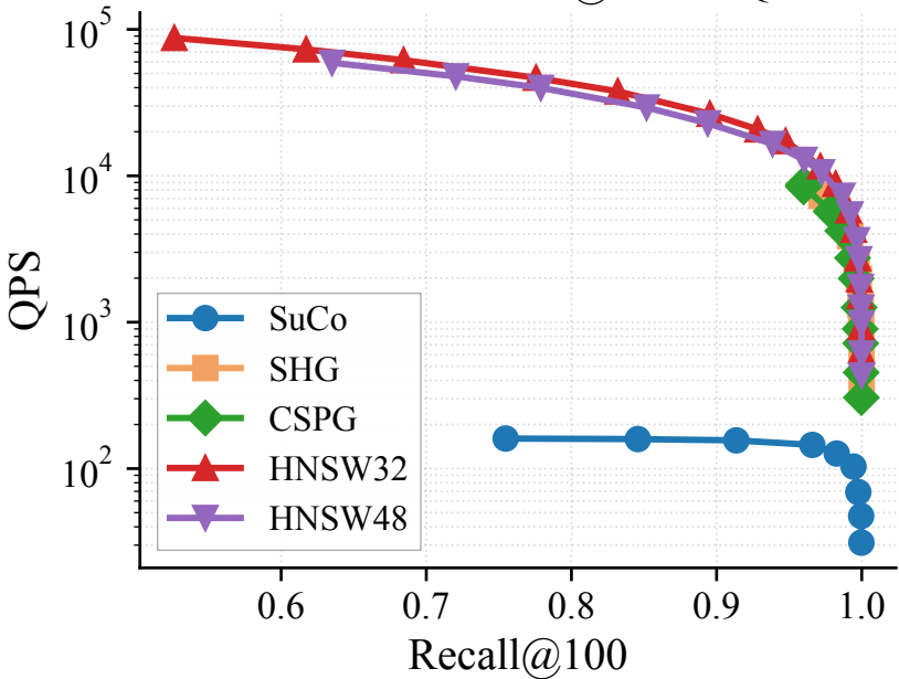
SIFT10M — Recall@100 vs QPS
