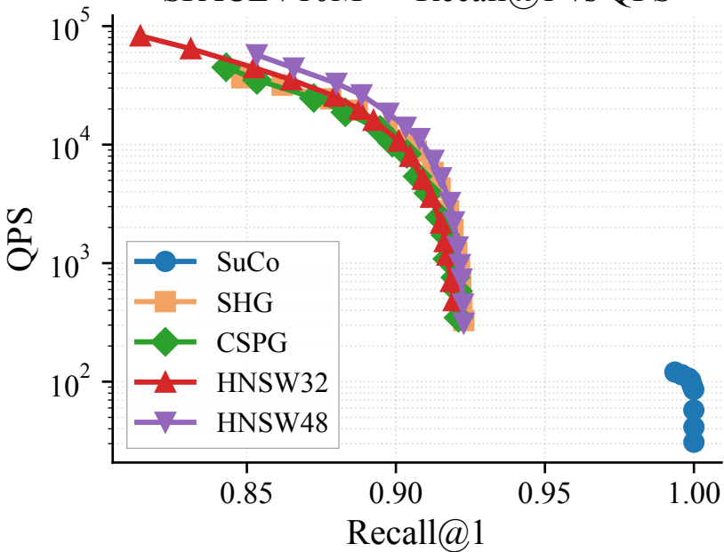
SPACEV10M — Recall@1 vs QPS
