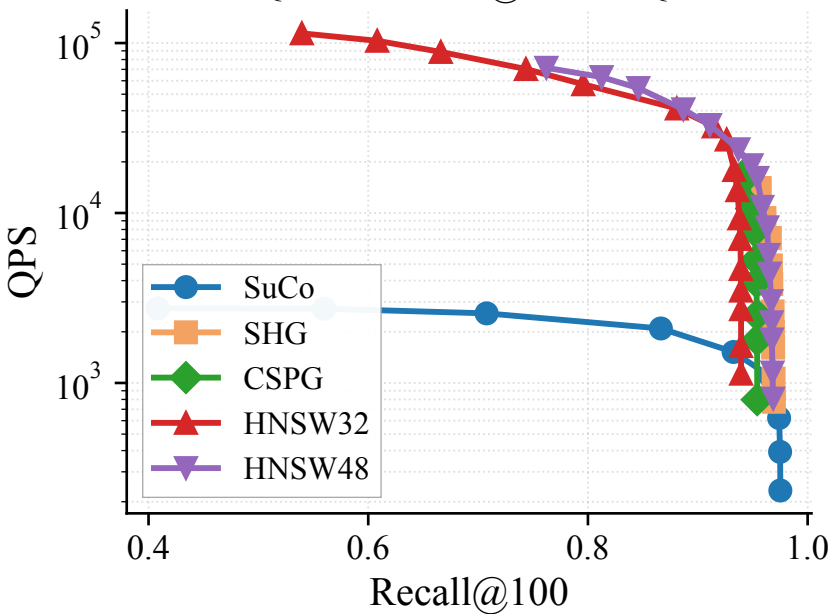
UQ-V — Recall@100 vs QPS
