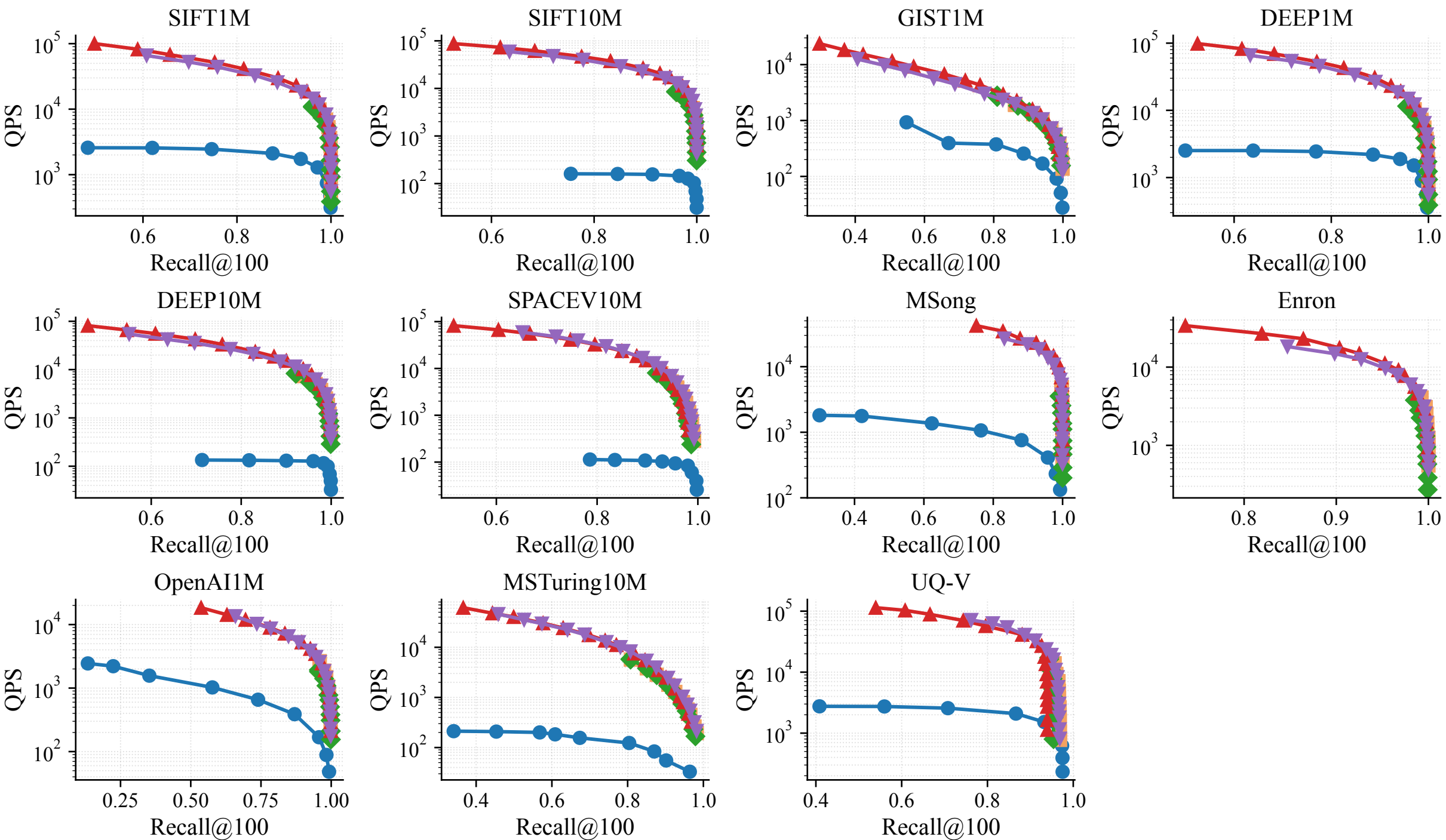
QPS vs Recall@100 — all datasets
