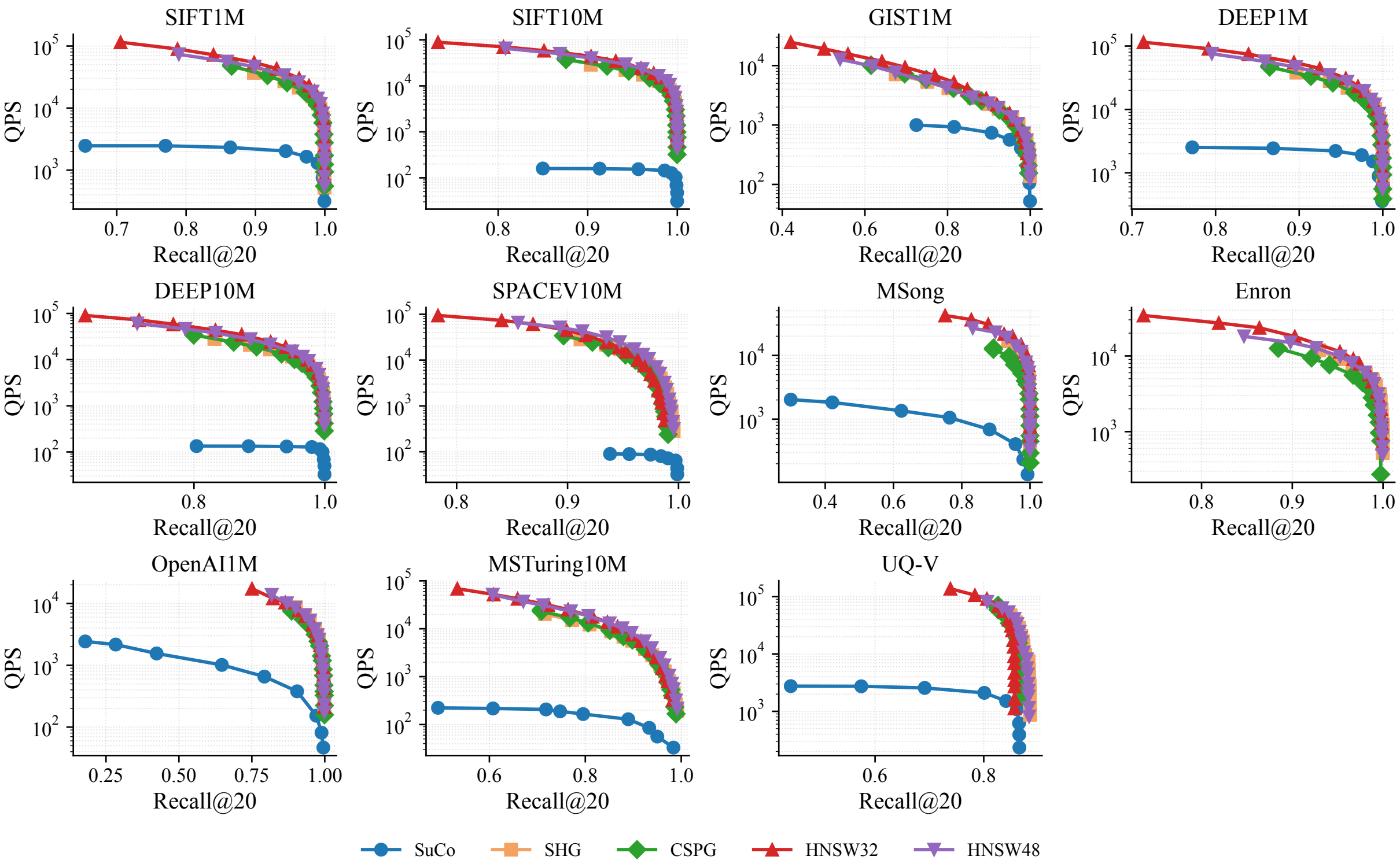
QPS vs Recall@20 — all datasets
