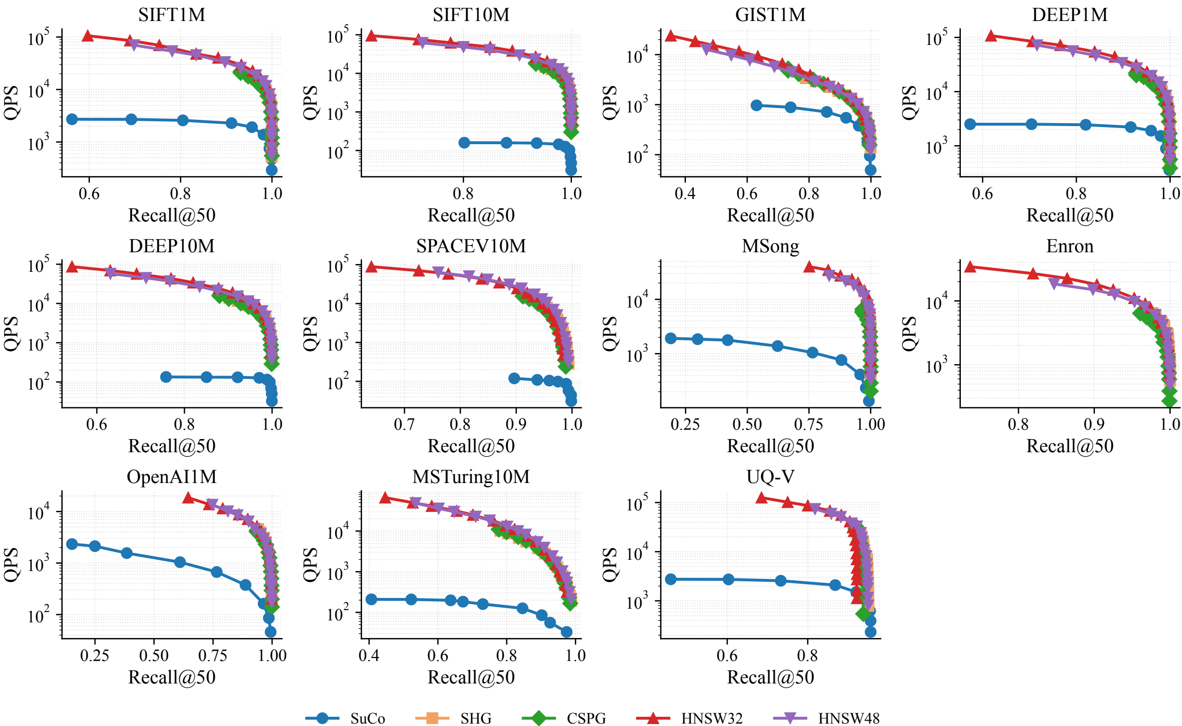
QPS vs Recall@50 — all datasets
