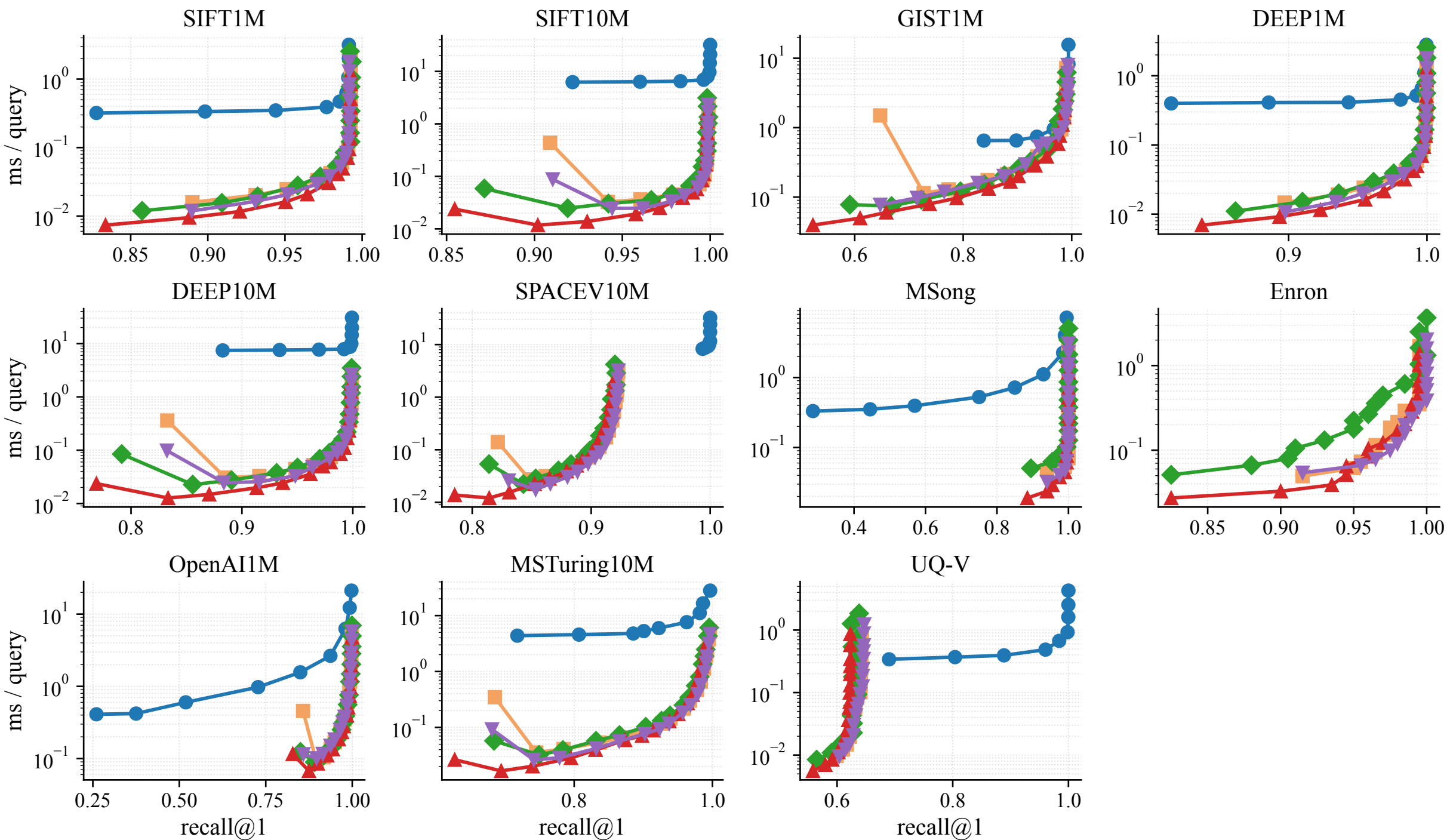
ms/query vs recall@1 (log-y)
