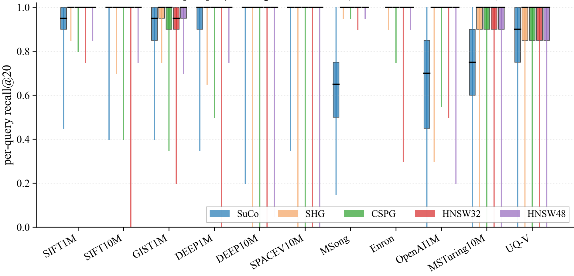
Robustness — per-query recall@20 distribution (min · 25–75% · median · max)
