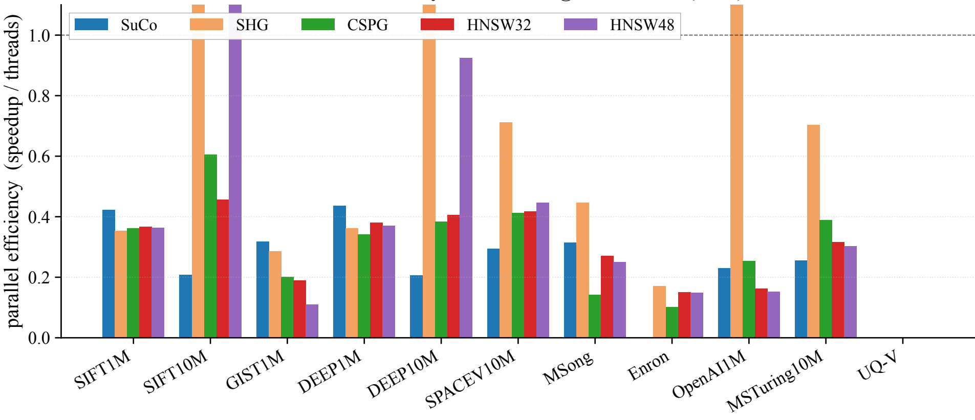
Parallel efficiency at 16 threads @ recall \geq 0.90 (k=10)
