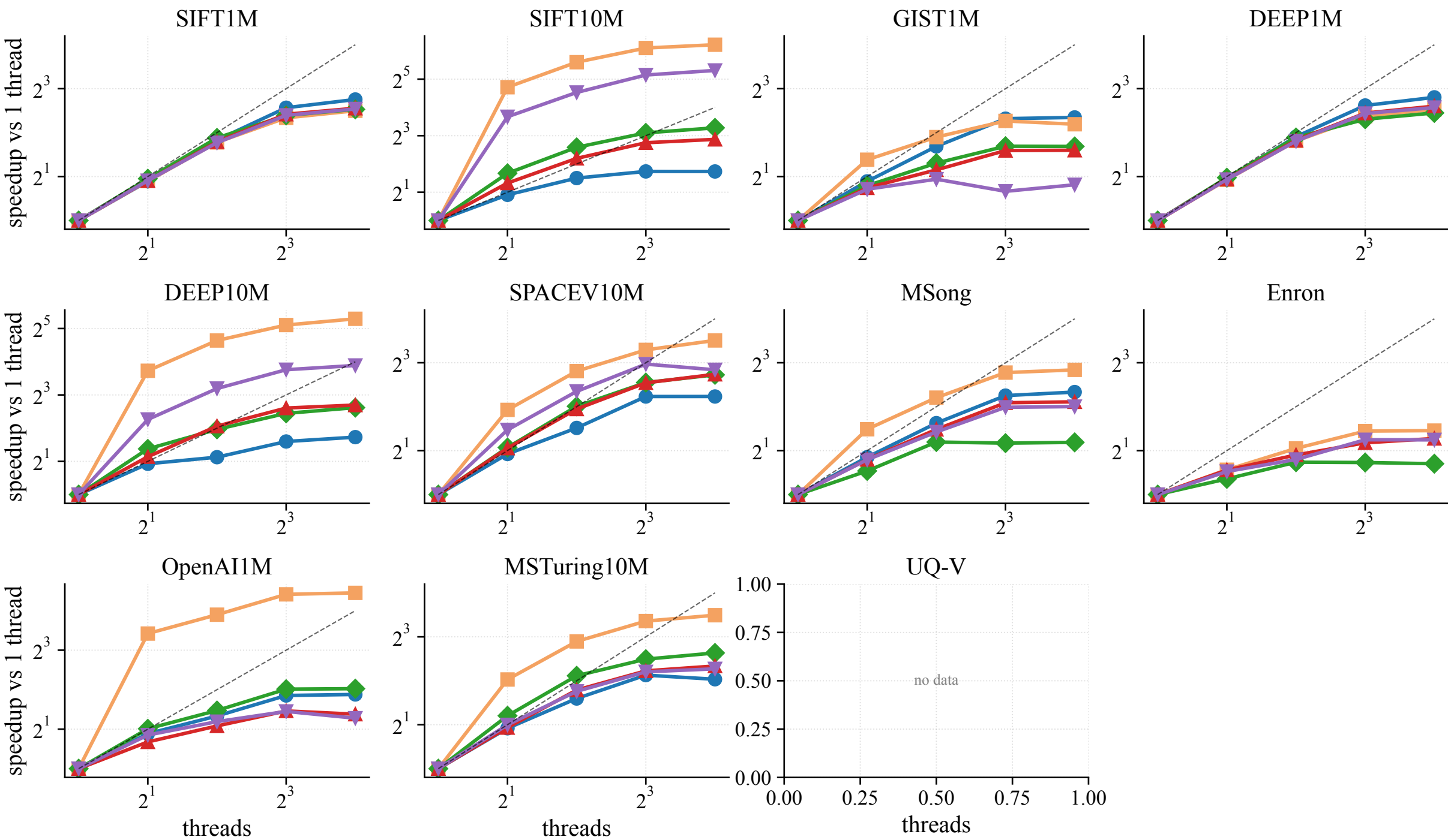
Thread-scaling: speedup vs 1 thread @ recall \geq 0.90 (k=10)
