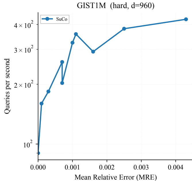
MRE vs QPS: 1M-scale datasets (SuCo)
