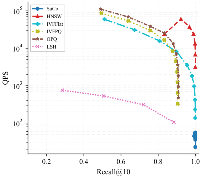
SIFT10M (easy, d=128)
