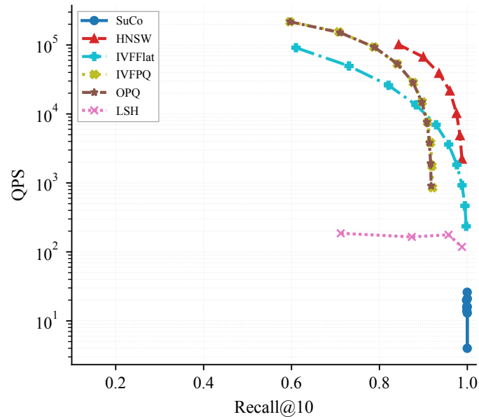
SpaceV10M (hard, d=100)
