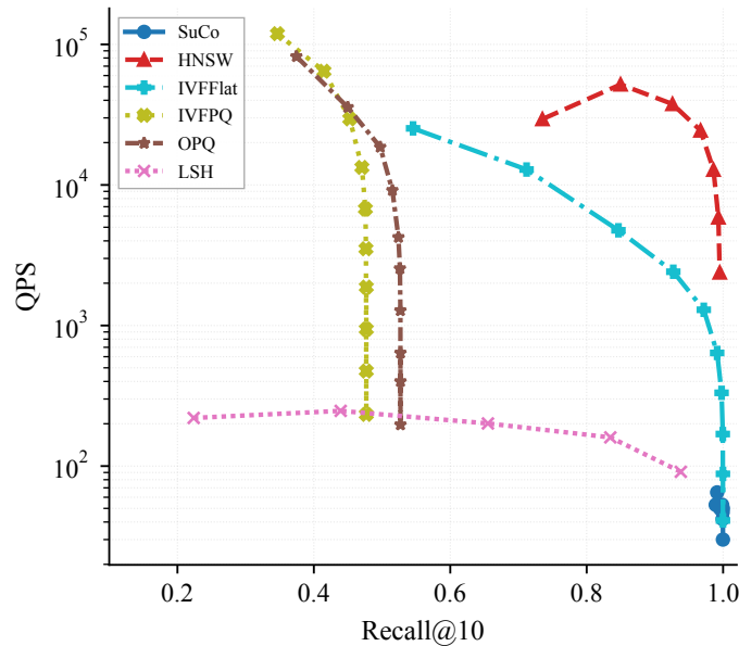
Deep10M (easy, d=96)
