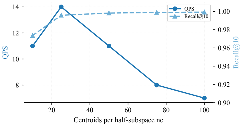
(c) Query perf vs nc (SIFT10M)
