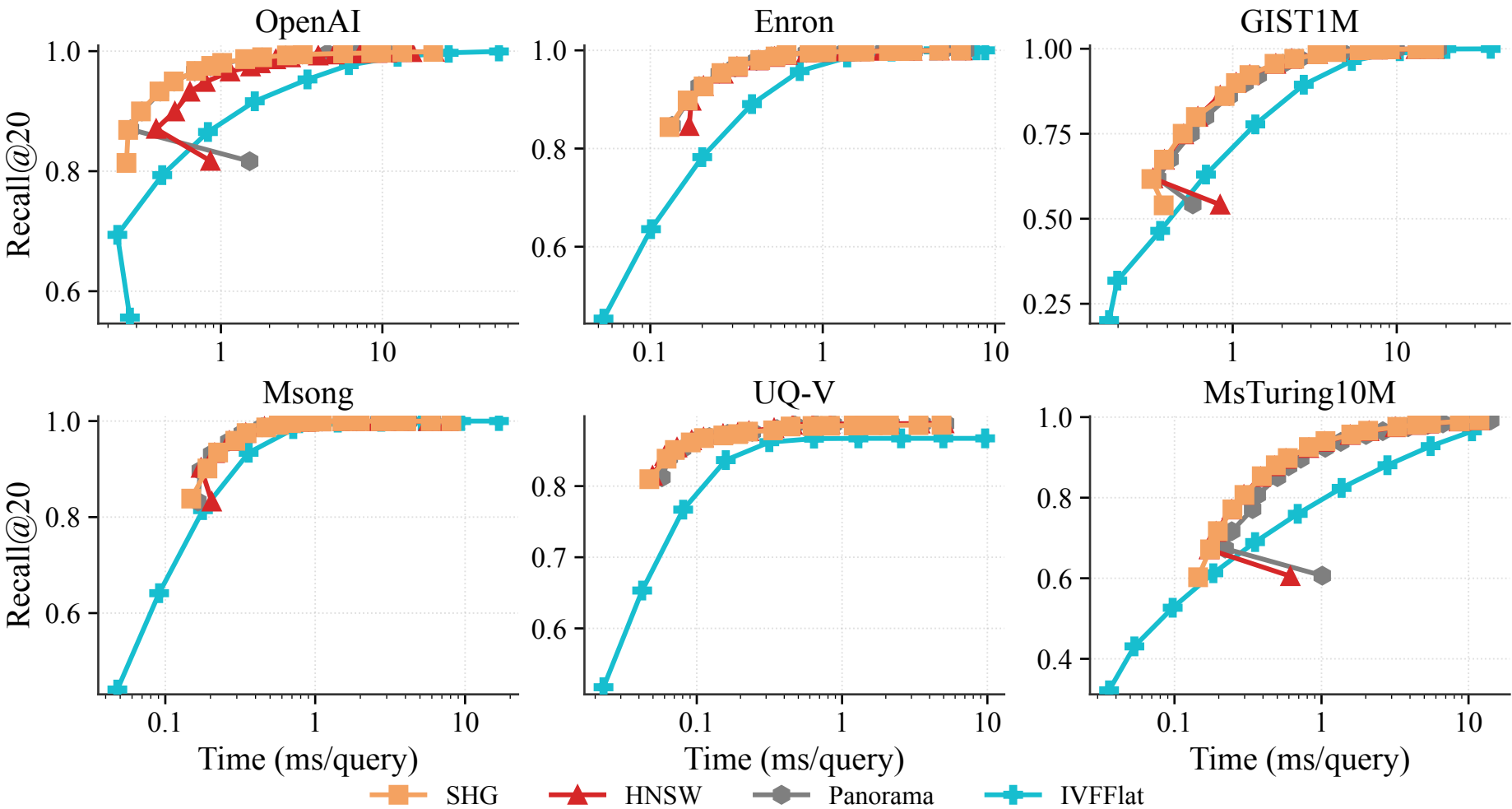
Recall@20 vs query time
