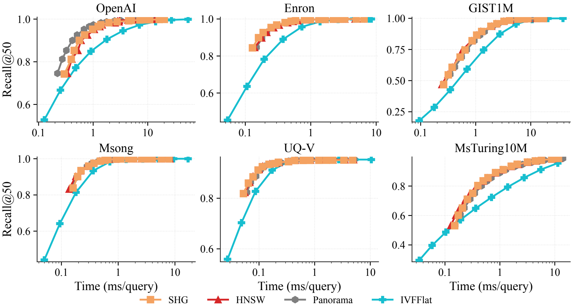
Recall@50 vs query time
