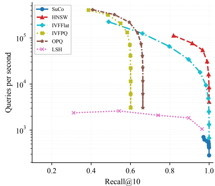
Deep1M (easy, d=96)
