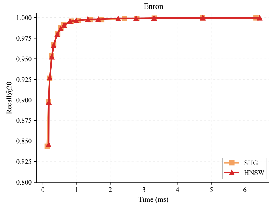
SHG vs HNSW — Recall vs Query Time (k=20)
