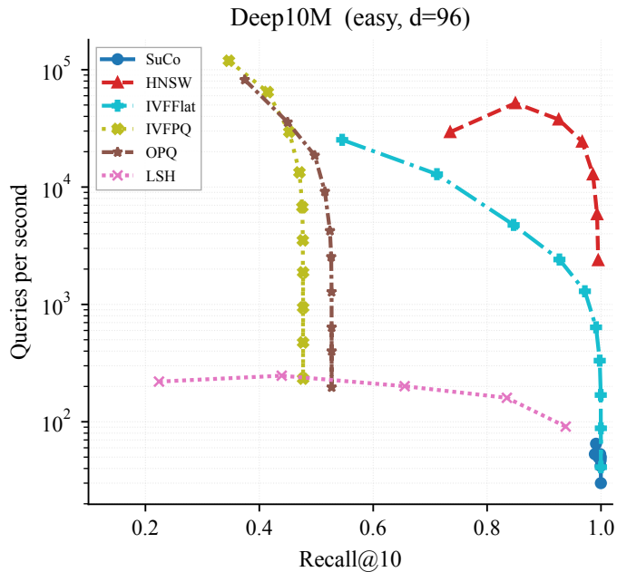
Recall@10 vs QPS: 10M-scale datasets
