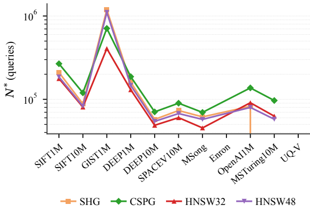
Build-plus-query crossover against SuCo
