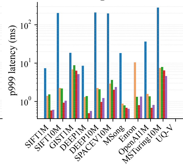
P999 @ recall 0.95
