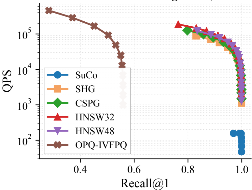
DEEP10M — Recall@1 vs QPS
