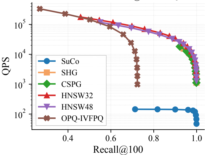
DEEP10M — Recall@100 vs QPS
