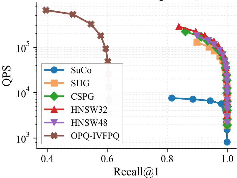
DEEP1M — Recall@1 vs QPS
