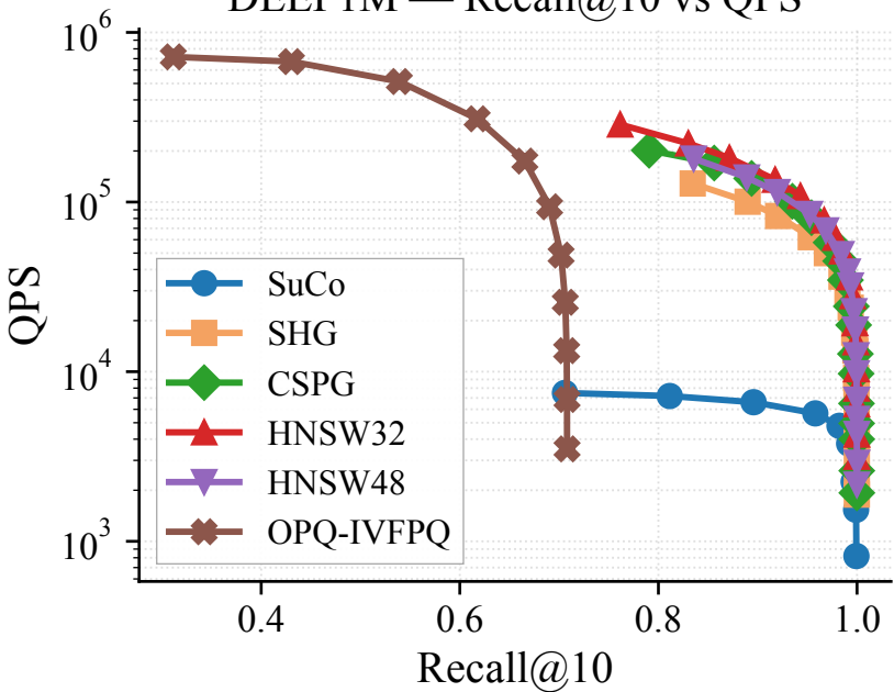
DEEP1M — Recall@10 vs QPS
